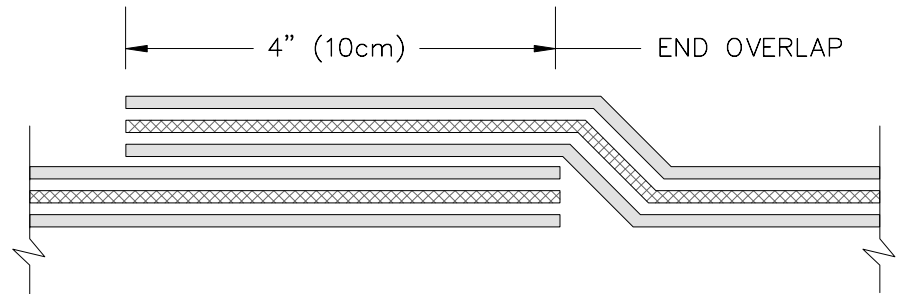
END OVERLAP DIMENSIONS FOR LIQUID APPLIED MEMBRANES ARE FOUR INCHES.
