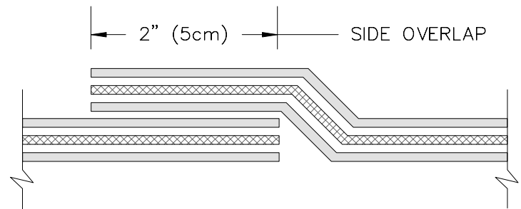
SIDE OVERLAP DIMENSIONS FOR LIQUID APPLIED MEMBRANES ARE TWO INCHES.
