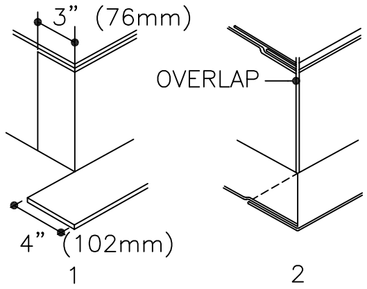
FIRST MEMBRANE FLASHING PLY
