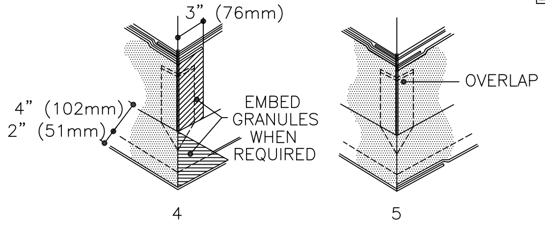
APPROVED CAP MEMBRANE FLASHING PLY
