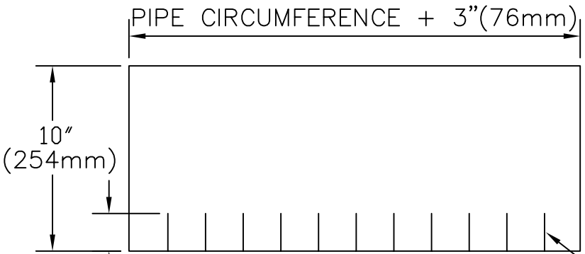
VERTICAL BASE MEMBRANE FLASHING WRAP SECOND CUT
