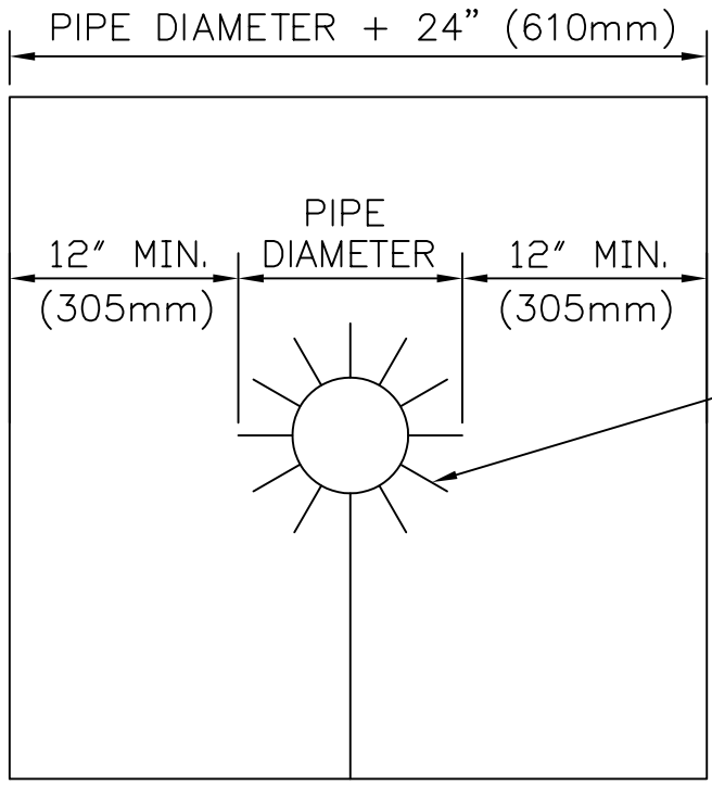
FIRST MEMBRANE FLASHING PLY FIRST CUT TARGET
