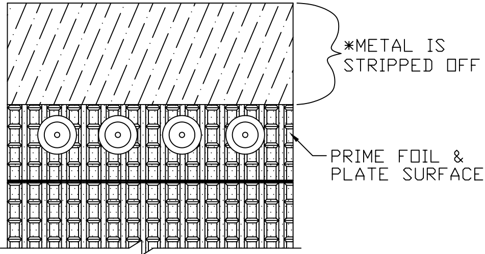
TOP VIEW
