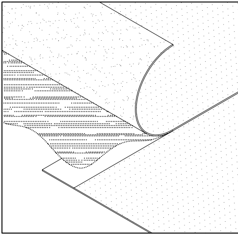
FOR ASPHALT APPLIED MEMBRANE, TAKE CAUTION WITH ASPHALT GETTING ONTO THE SOPRASTAR
