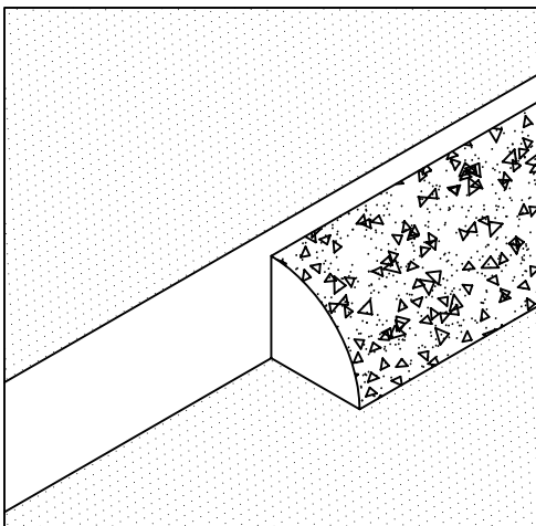
UPON COMPLETION OF THE SEAM, A SOPRASTAR CHIPS MAY BE APPLIED TO THE EXCESS LAP SEALANT OR BLEED-OUT.
