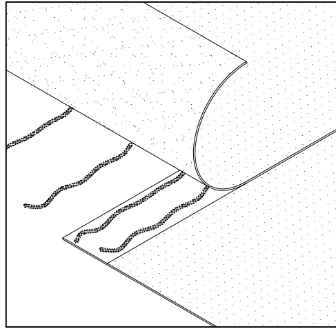
FOR RIBBON APPLIED ADHESIVES, APPLY ADHESIVE RIBBONS ONTO THE LAP
